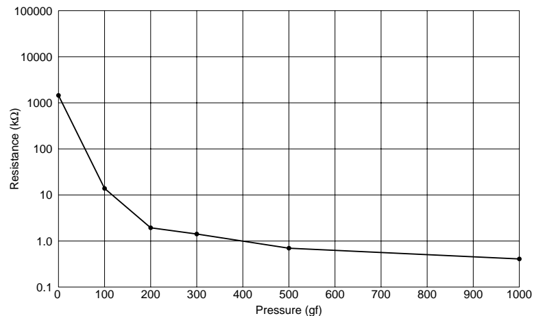
Pressure vs Resistance (average from 3 samples)
